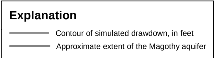
Figure 12c. Simulated drawdown in the Magothy aquifer, 2002 to 2030, based on Scenario 5b.
