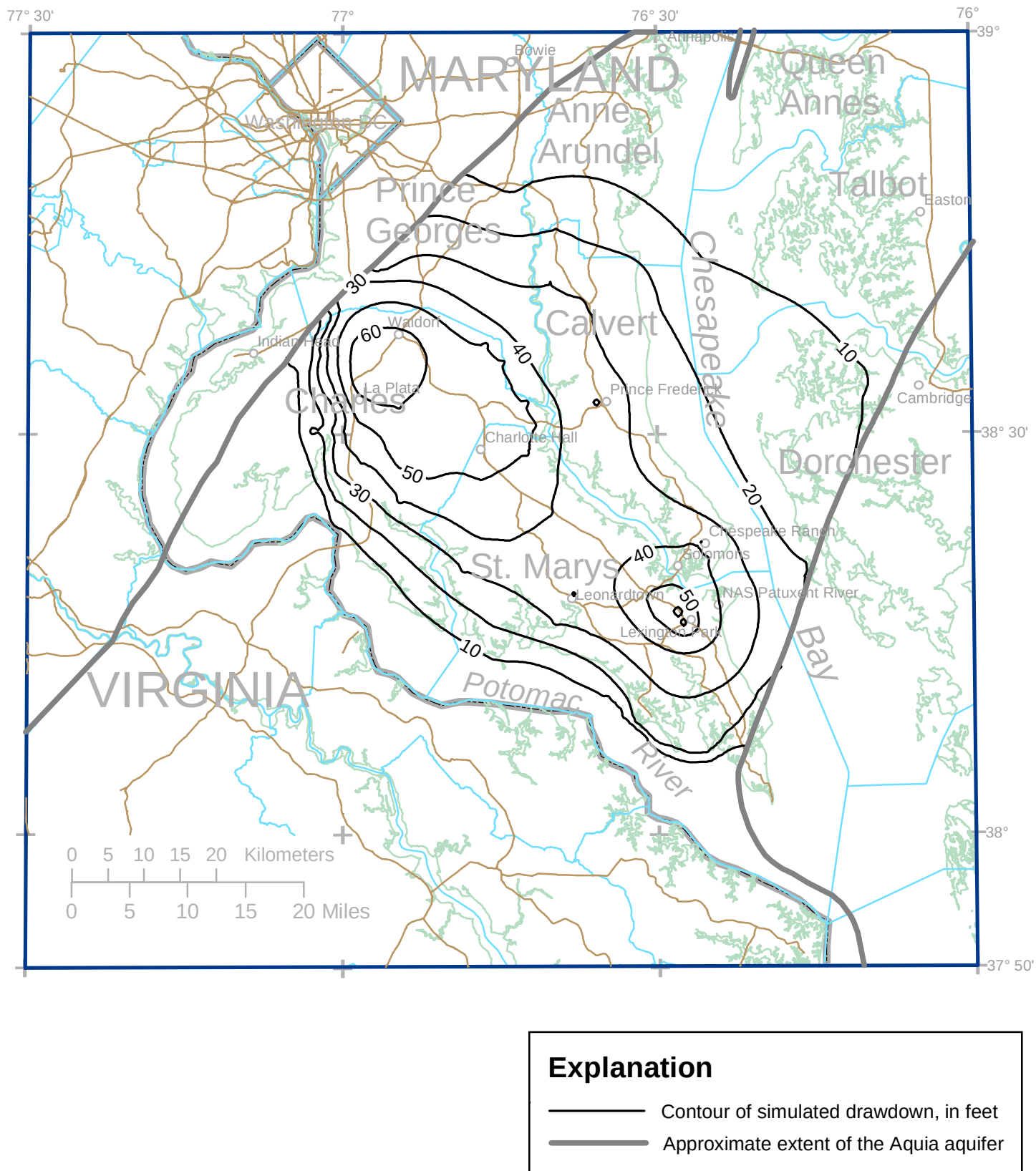
Figure 10b. Simulated drawdown in the Aquia aquifer, 2002 to 2030, based on Scenario 1.
