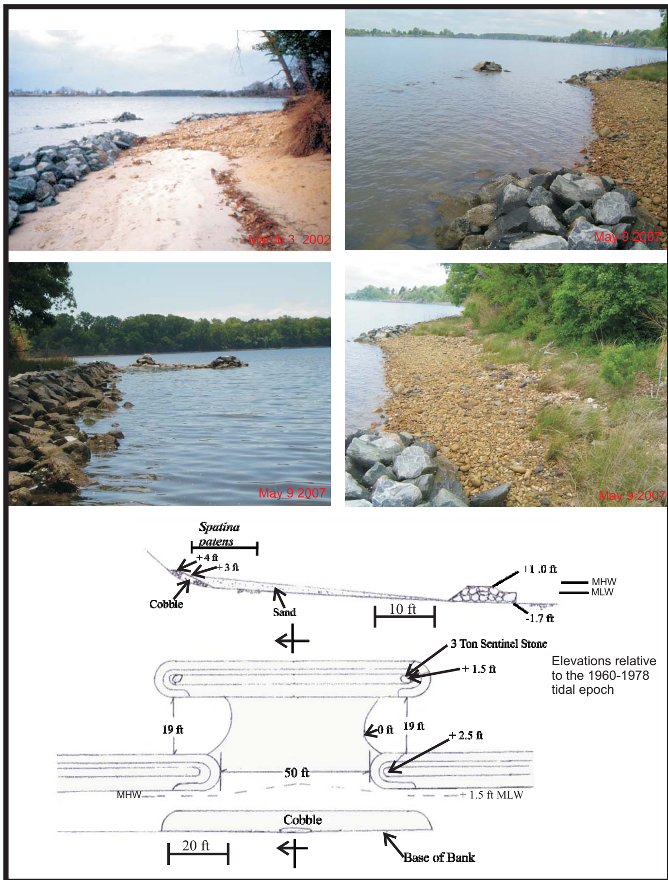
Figure 2-9. Photos showing Window 8 post construction in 2002 and in 2007. Window 8 is a Type III window or vent along Site 1 with a cobble backshore and an offshore low breakwater as shown in the planform and cross-sectional design.
