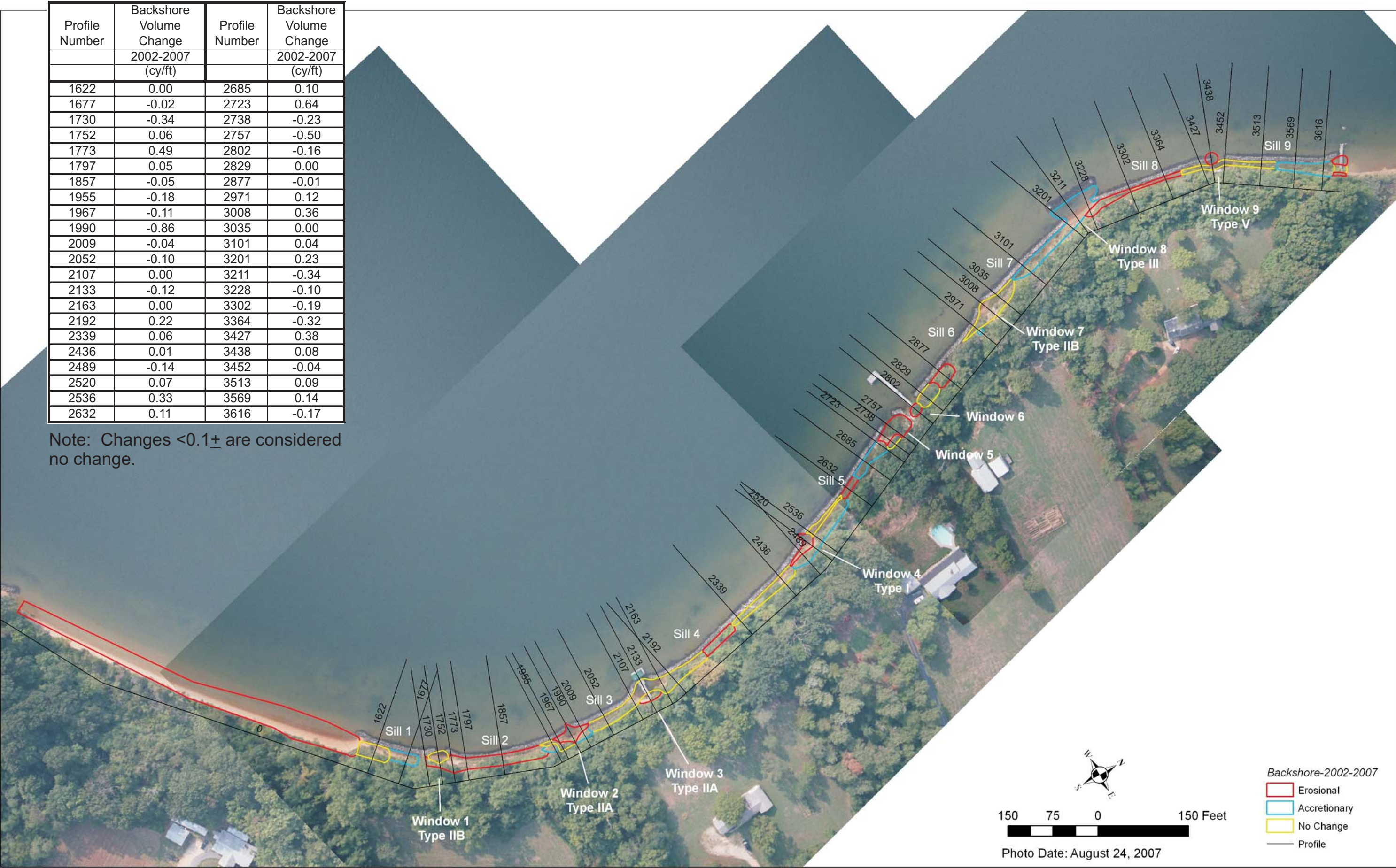
Figure 2-11. Map showing the change along the backshore planting terrace between 2002 and 2007 based on profile data. Also shown are profile lines and volume change in cy/ft associated with each profile.
