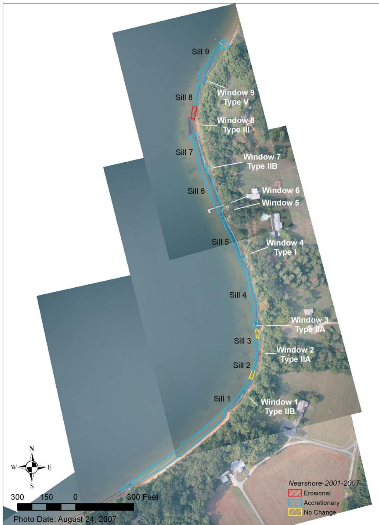
Figure 2-12. Map depicting changes in the nearshore between preinstallation (2001) and recently (2007).
